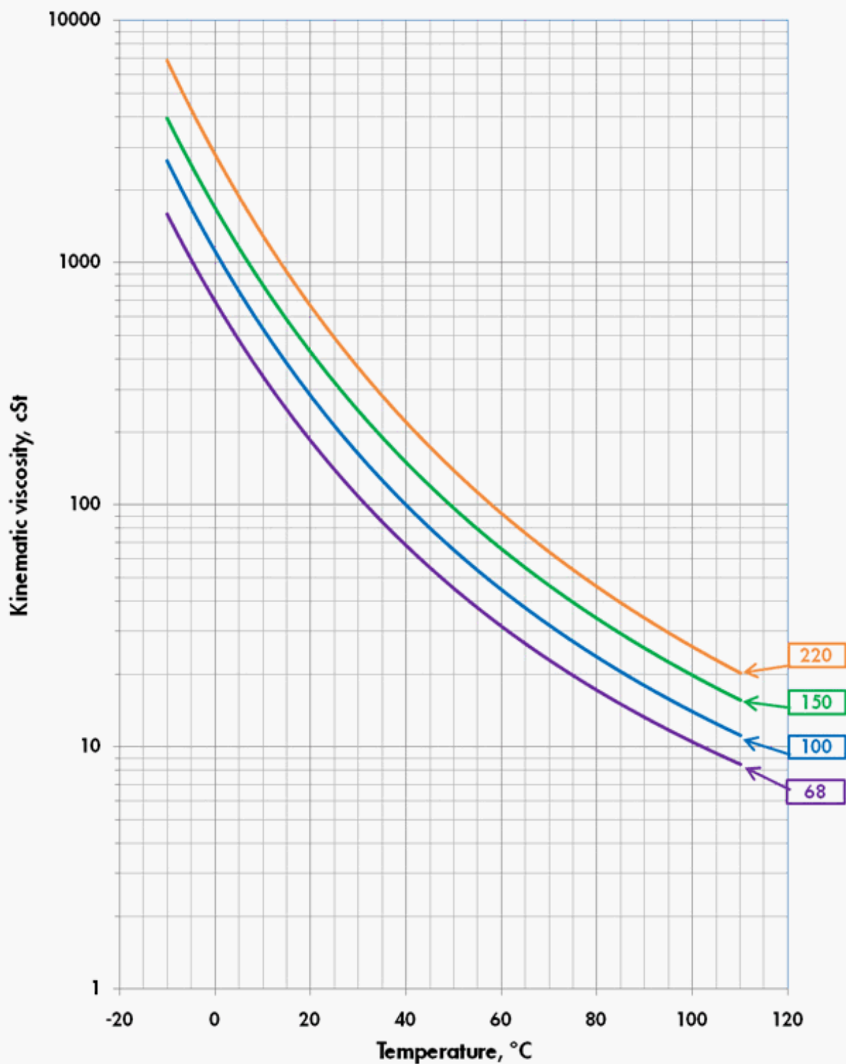
Viscosity - Temperature Diagram for Shell Morlina S4 B
